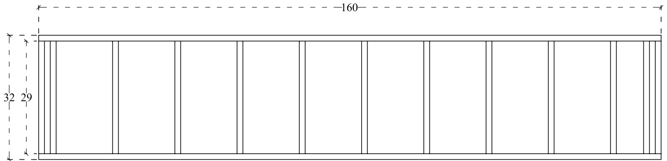
South wall frame. 2x4 nominal studs
