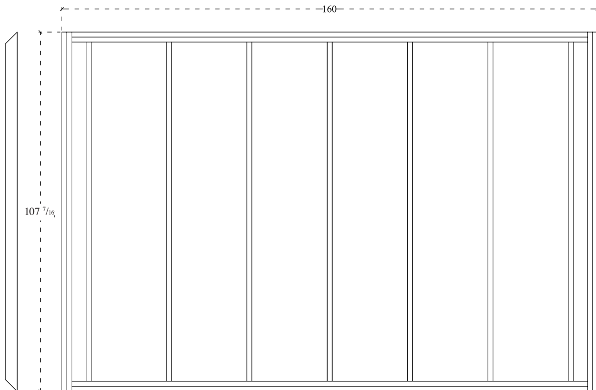
Frame - Roof 2x4 framing
