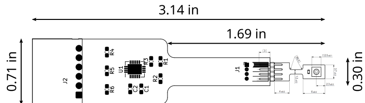
Remote Rev 4 Replace RJ-45 with 6-pin Molex SL
