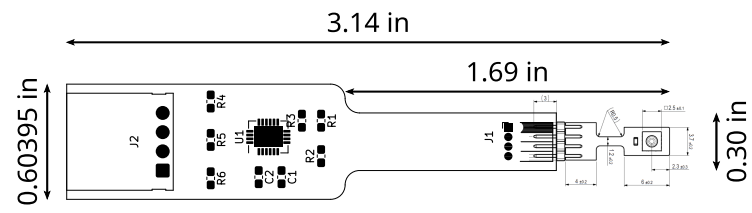
Remote Rev 5 Replace RJ-45 with 4-pin Molex SL
