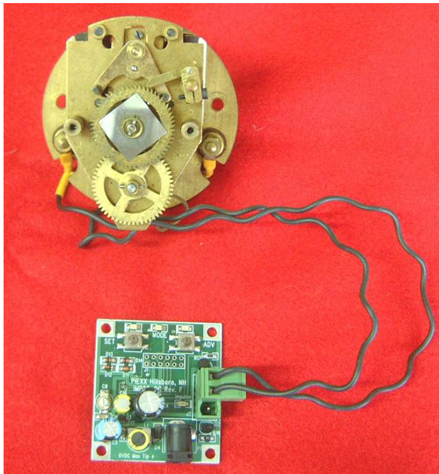
IMP-22 Connected to a Brille Movement. Brille uses the same connections as a Gents.
